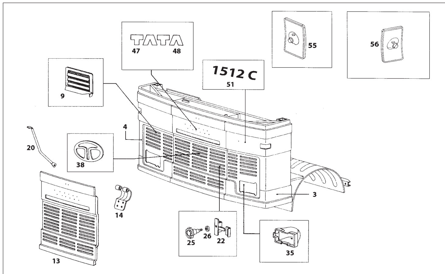
INTERNAL AND EXTERNAL FITMENTS (COWL WITH FACE)
