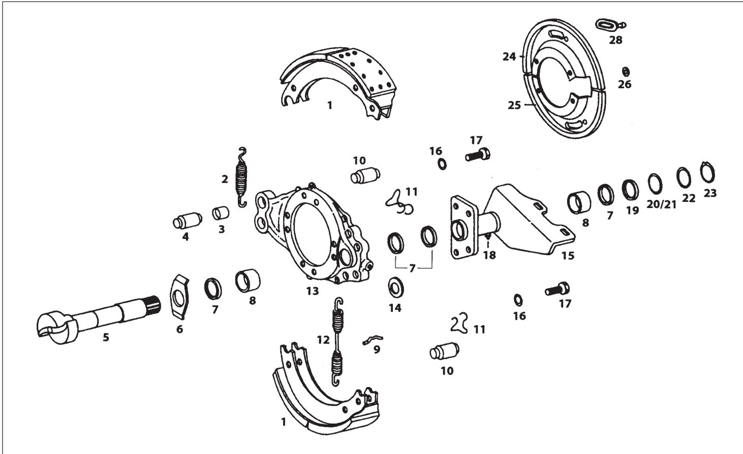
FRONT WHEEL BRAKE (M/S KTMS)
