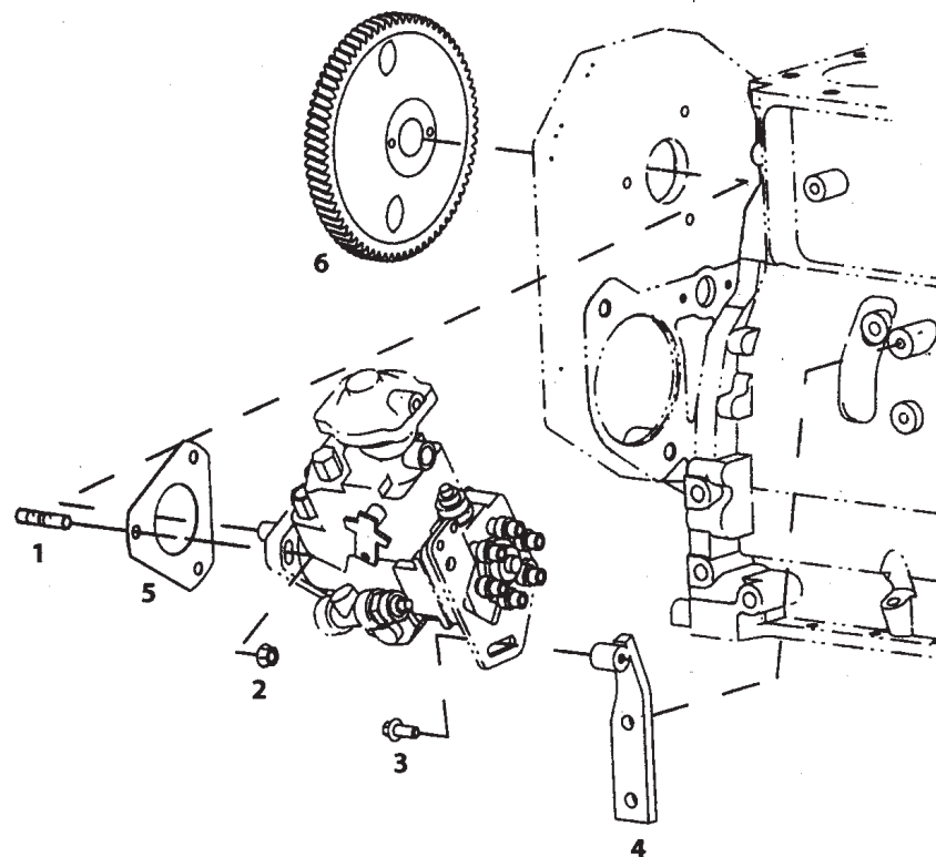
FUEL PUMP COUPLING
