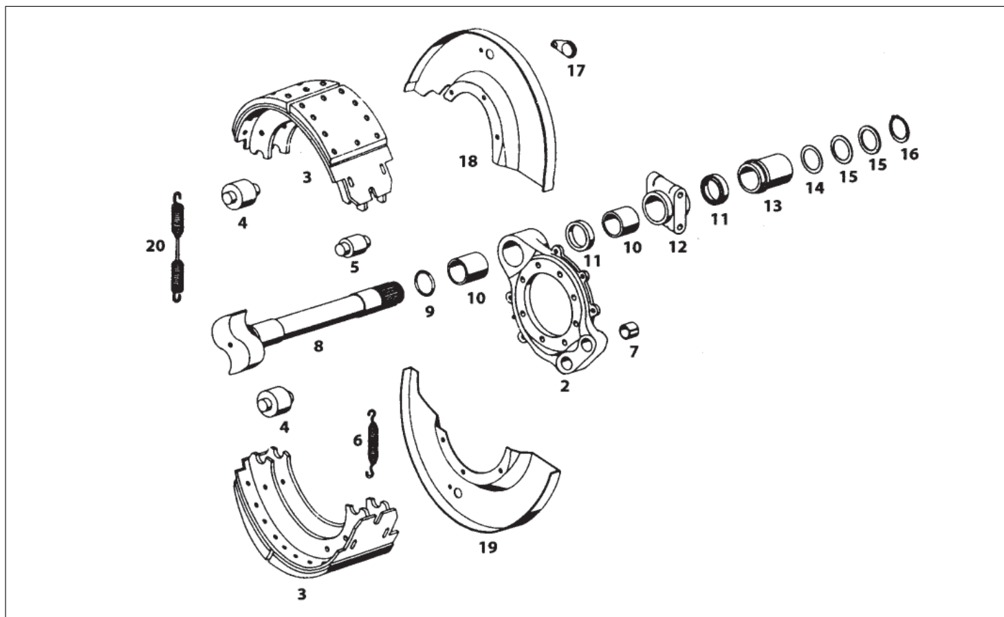
REAR WHEEL BRAKE (BIL)-LPO
