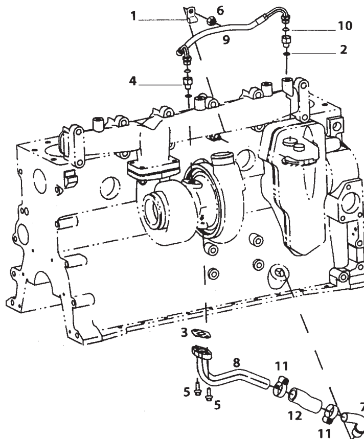
TURBOCHARGER PLUMBING
