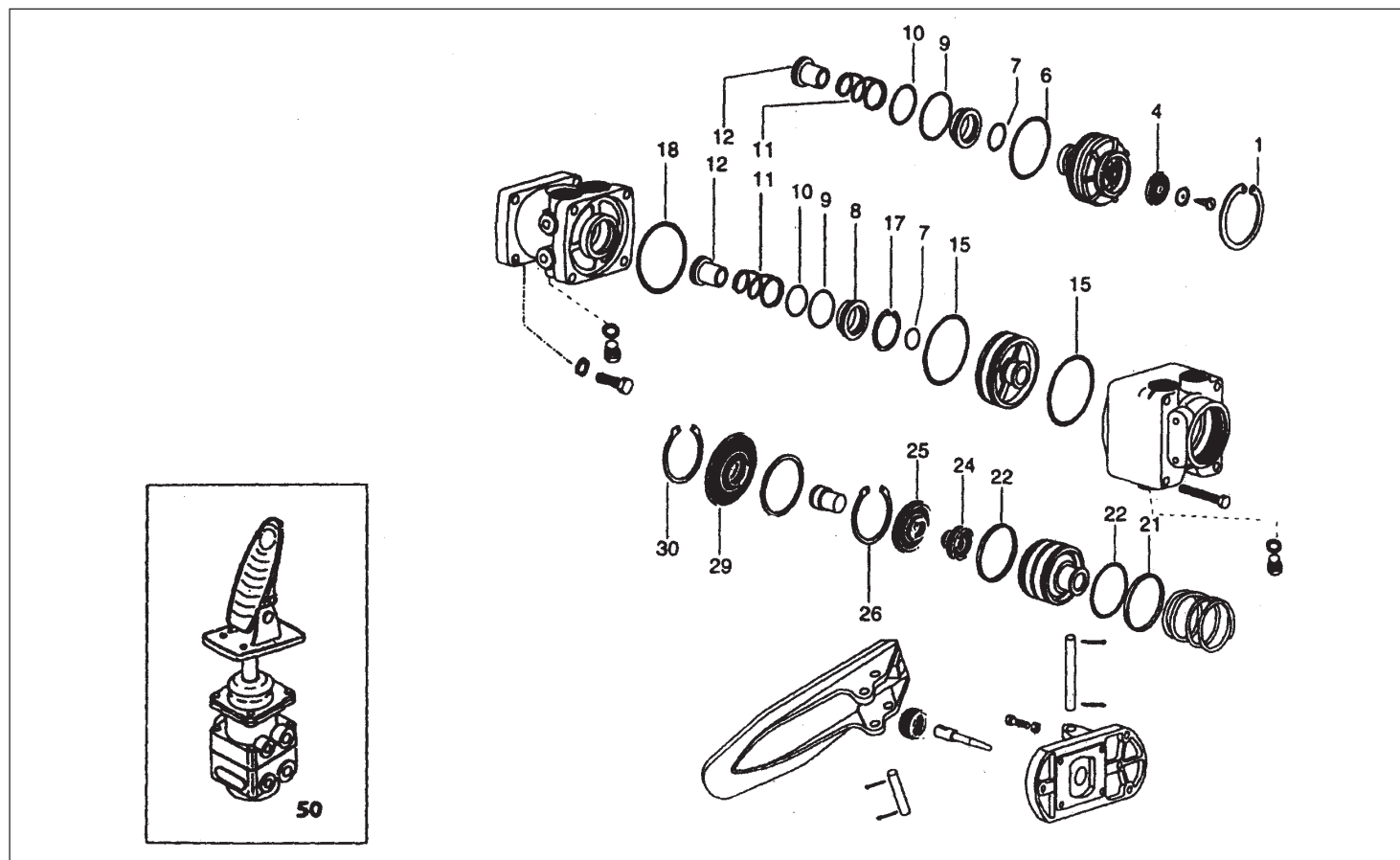
DUAL BRAKE VALVE (LPO)
