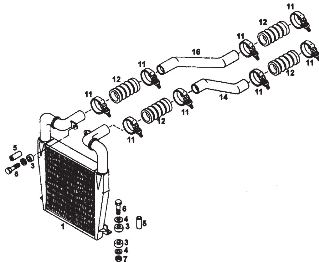
INTERCOOLER AND INTERCOOLER CONNECTION
