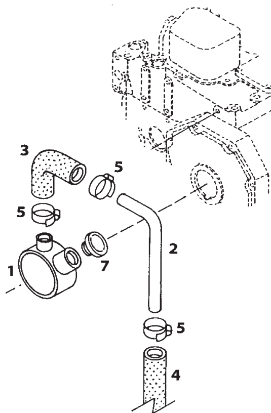
OIL FILL LOCATION
