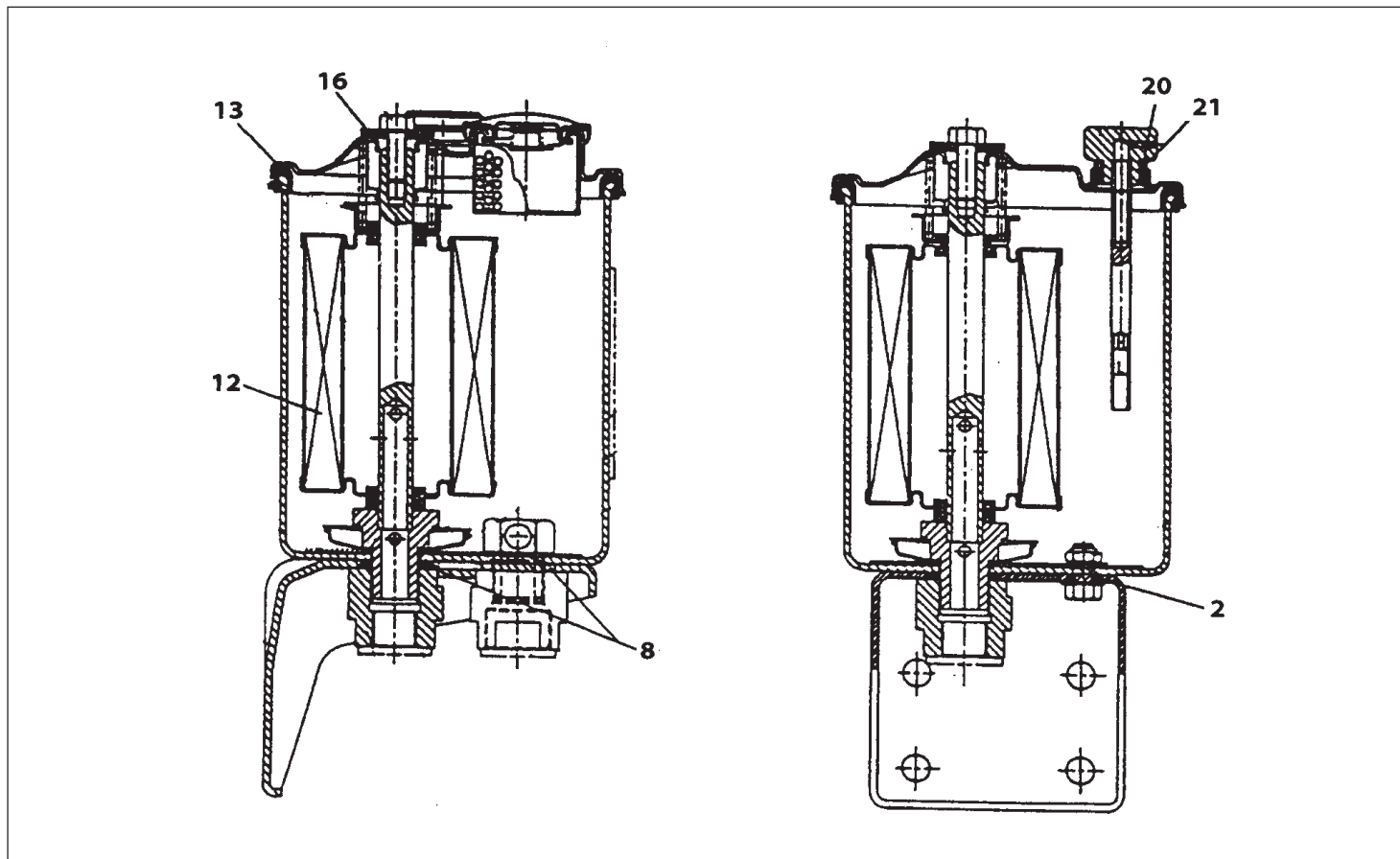
HYDRAULIC TANK (RANE)
