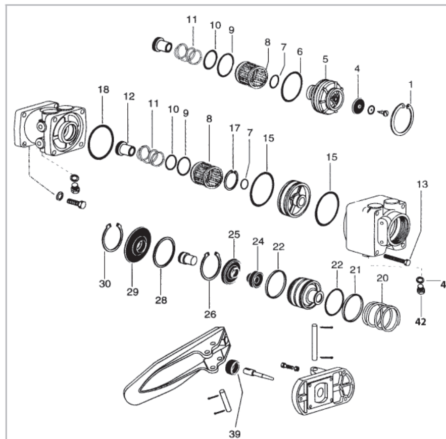
DUAL BRAKE VALVE (LP)
