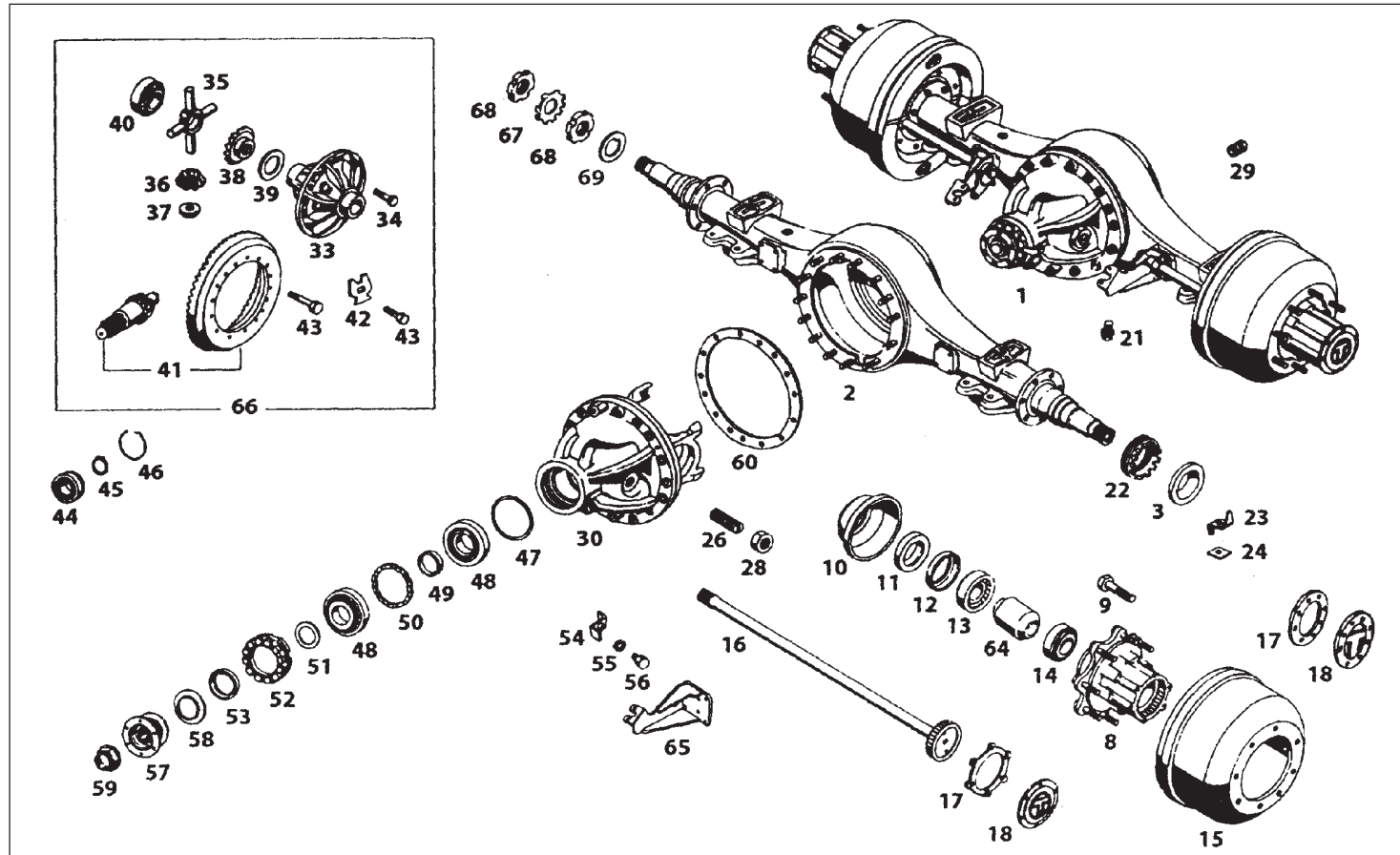
REAR AXLE(108-RR)
