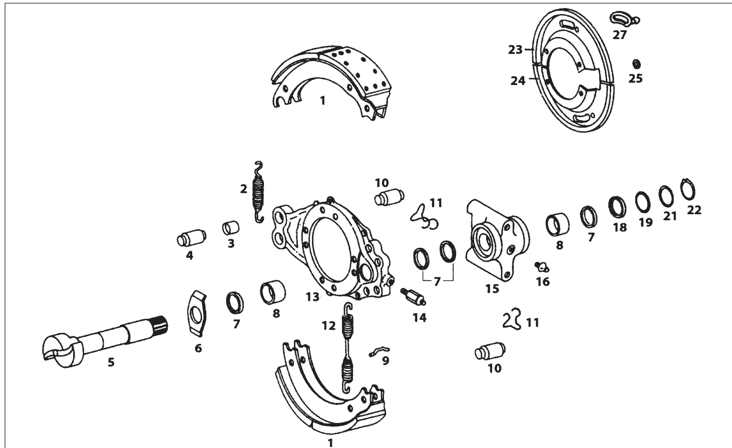
REAR WHEEL BRAKE (M/S KTMS)-LP
