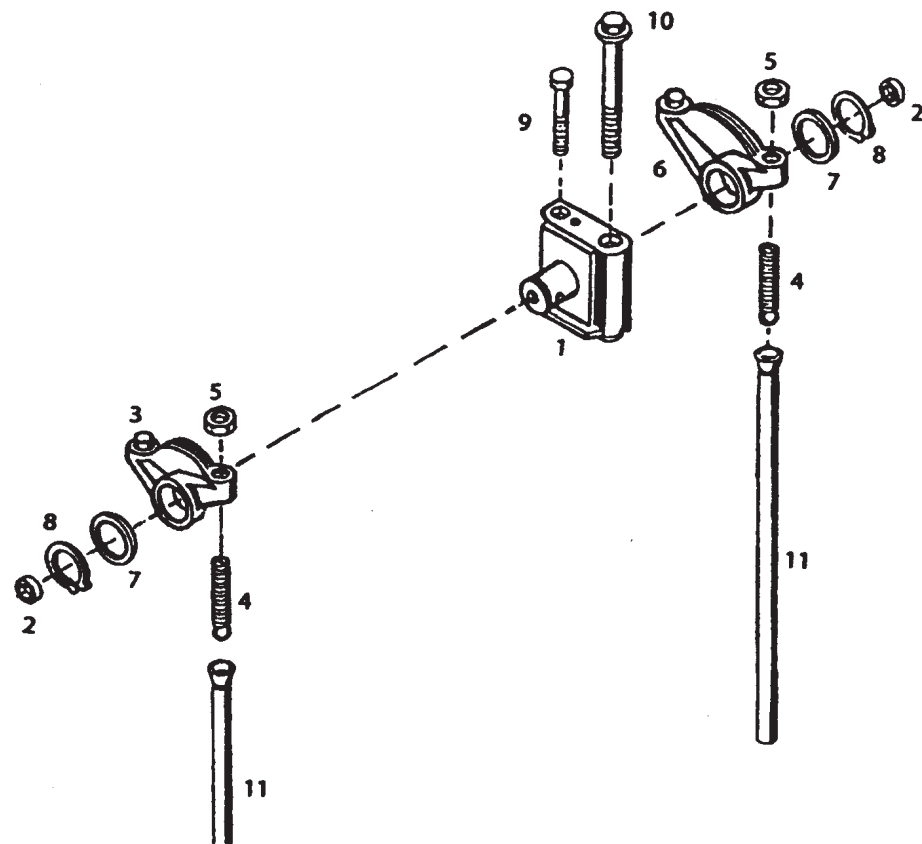
ROCKER LEVER
