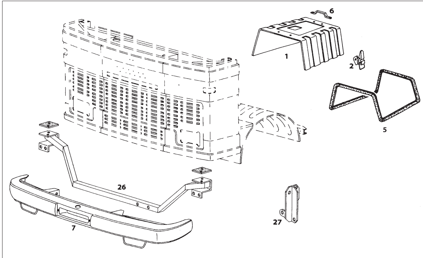
ENGINE HOOD, BUMPER AND ANTI SAGGING BAR
