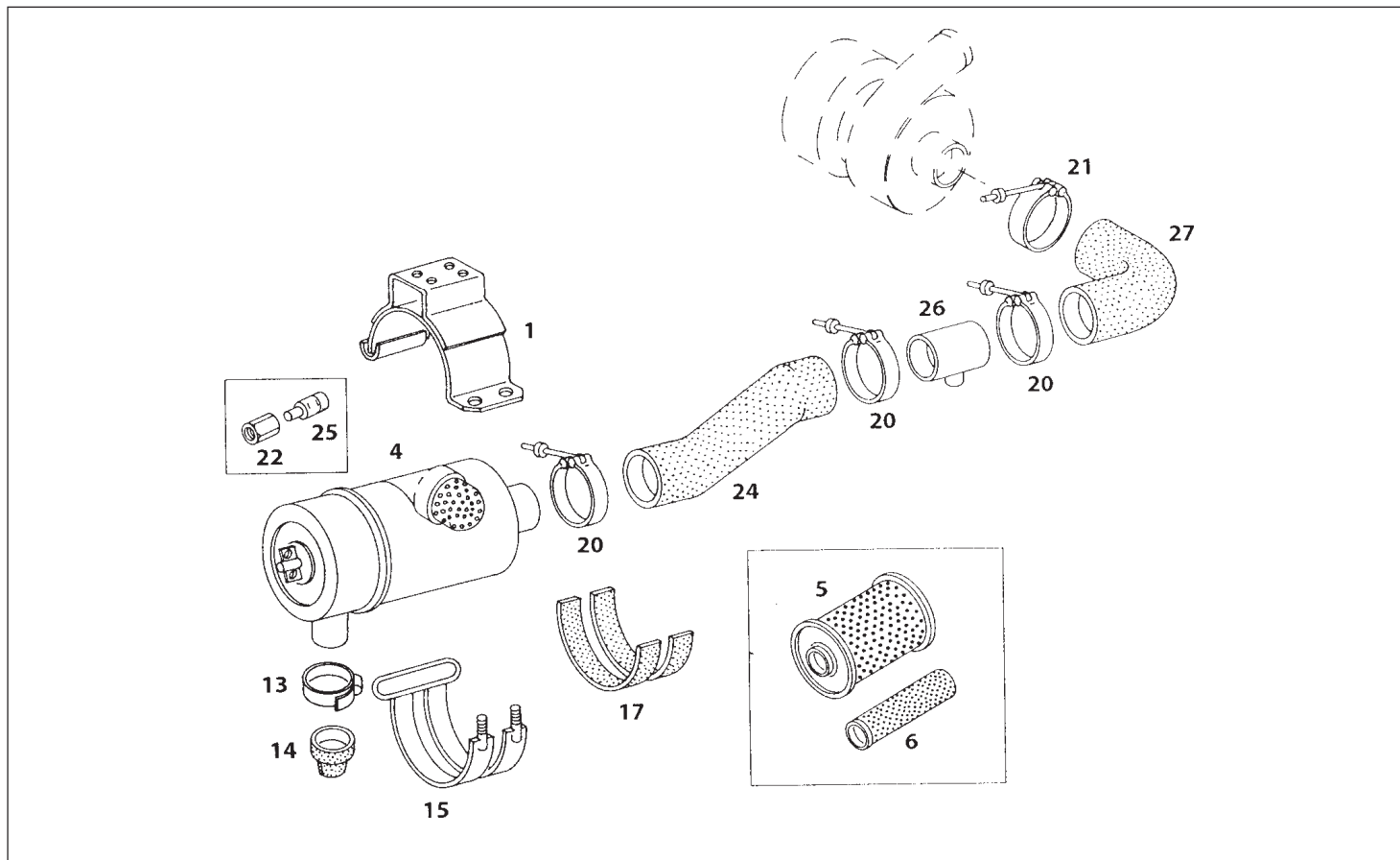
AIR FILTER (LPO)
