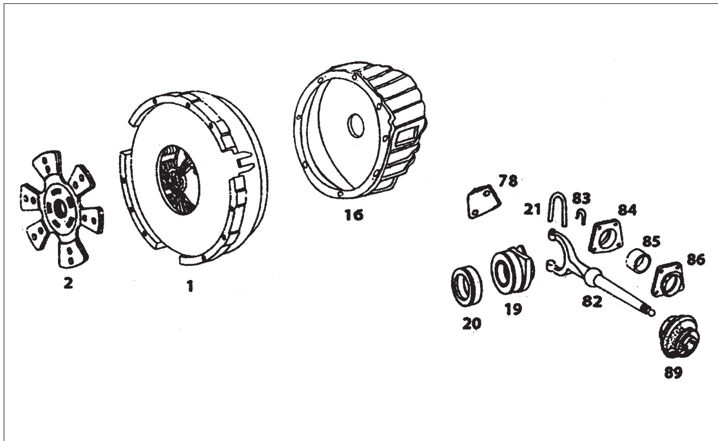
CLUTCH 330 DIA. (COIL TYPE)
